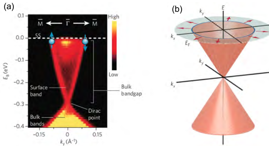
Figure 2.2: Surface states in the topological insulator \text{Bi}_2\text{Se}_3 . (a) Electronic band structure was obtained from angle-resolved photoemission spectroscopy (ARPES) experiment. E_B is the measured electron energy. \bar{\Gamma} , \bar{M} are the respective symbols for Brillouin-zone centre and Brillouin-zone boundary in the reciprocal space. Dirac point at \bar{\Gamma} is regarded as the proof for topological insulator. (b) Theoretical calculation of the electronic band structure of \text{Bi}_2\text{Se}_3 , showing the rotation of the spin degree of freedom (red arrows) as an electron (with energy E ) moves around the Fermi surface (taken from Ref.[25]).
