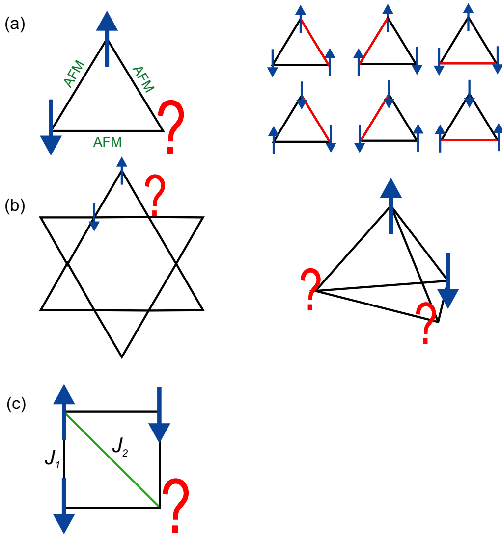
Figure 2.10: Magnetic frustrations in various lattices. (a) Geometry frustration in an equilateral triangle with antiferromagnetic Ising spins gives rise to six possible ground states. (b) A David' star with six triangles in the two dimensional (2D) kagomé lattice (left) and three dimensional (3D) tetrahedral lattice with four non-coplanar triangles (right). (c) In a square lattice with competing antiferromagnetic interactions of nearest-neighbour coupling J_1 and next-nearest-neighbour coupling J_2 of Ising spins, if the strength of J_1 and J_2 are comparable, a simple antiparallel arrangement of spins between all possible nearest-neighbour sites cannot be satisfied simultaneously.
