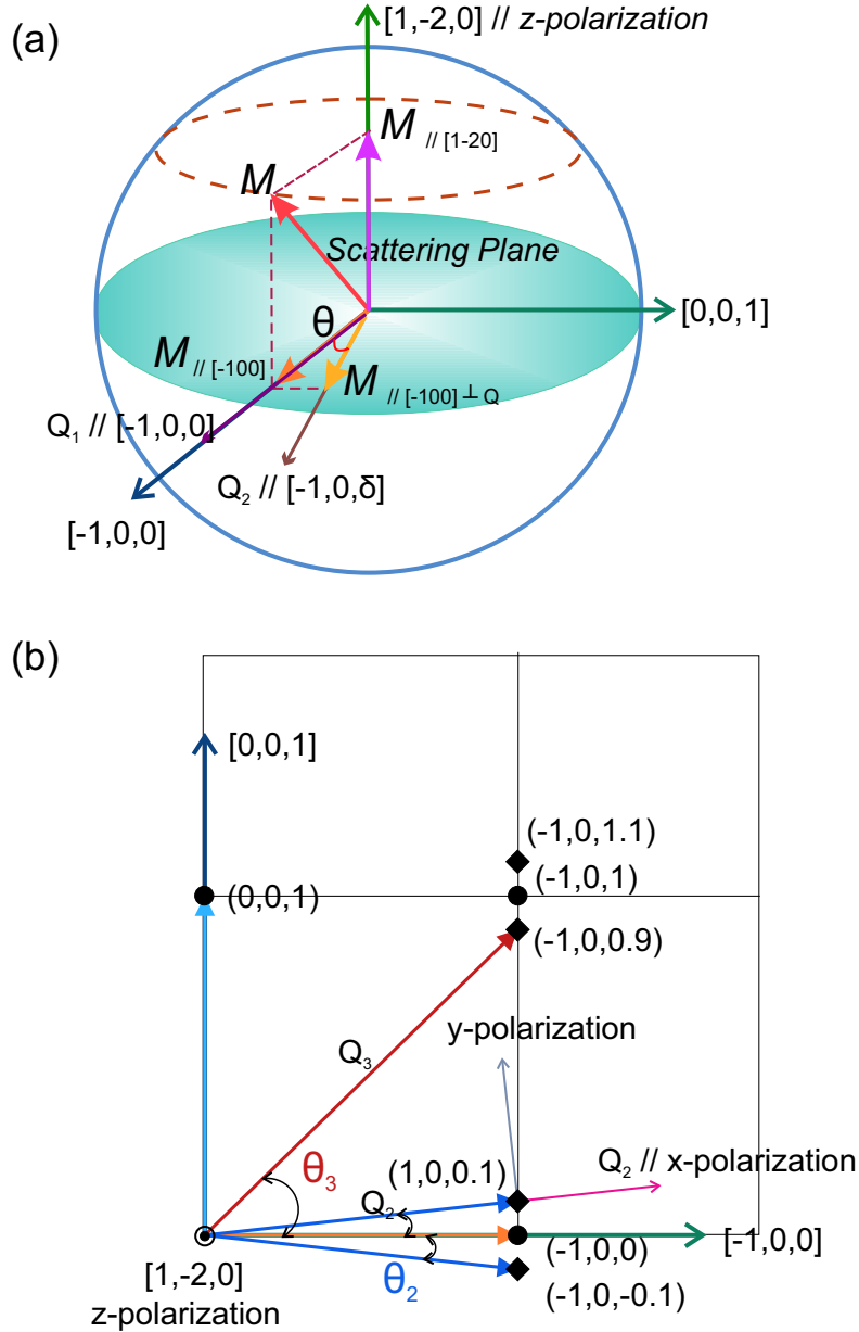
Figure 4.12: Scattering geometry of the experiments at DNS at MLZ. (a) The scattering plane is (h0l) plane where the magnetic moment M in (hk0) plane can be decomposed into M_{[1,\bar{2},0]} and M_{[\bar{1},0,0]} first. Then M_{[\bar{1},0,0]} can be further projected onto [0,0,1] direction M_{[\bar{1},0,0]\perp Q} . Q_1 is the scattering vector for the reflection [\bar{1},0,0] in crystallographic ab plane and Q_2 is the scattering vector for modulated reflections. \theta is the angle between scattering vector Q and (hk0) plane. (b) The (h0l) plane and the scattering vectors are depicted, where \theta is shown.
