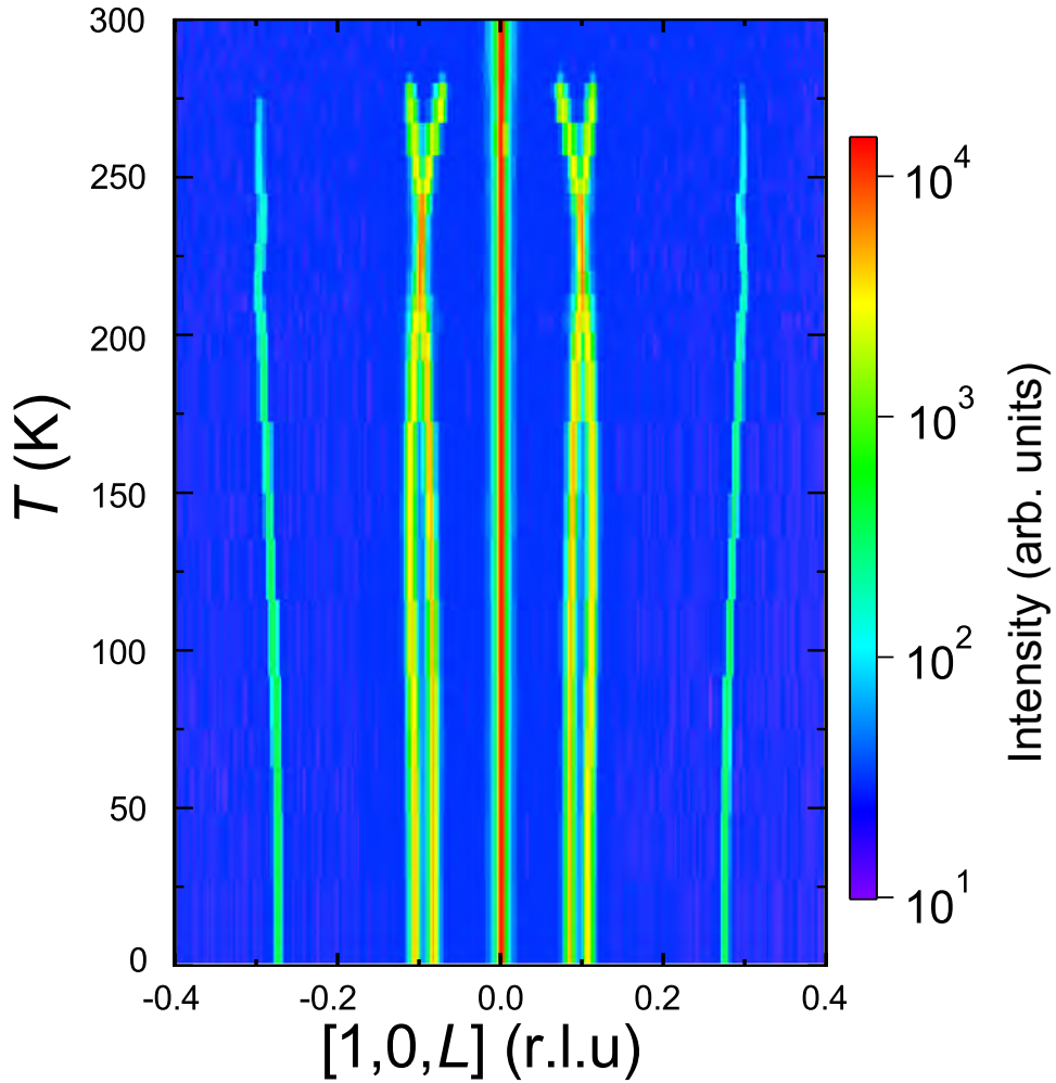
Figure 4.15: Contour map of temperature dependence of incommensurate phases in Mn_3Sn measured at the two-axis neutron diffractometer D23 at ILL.
