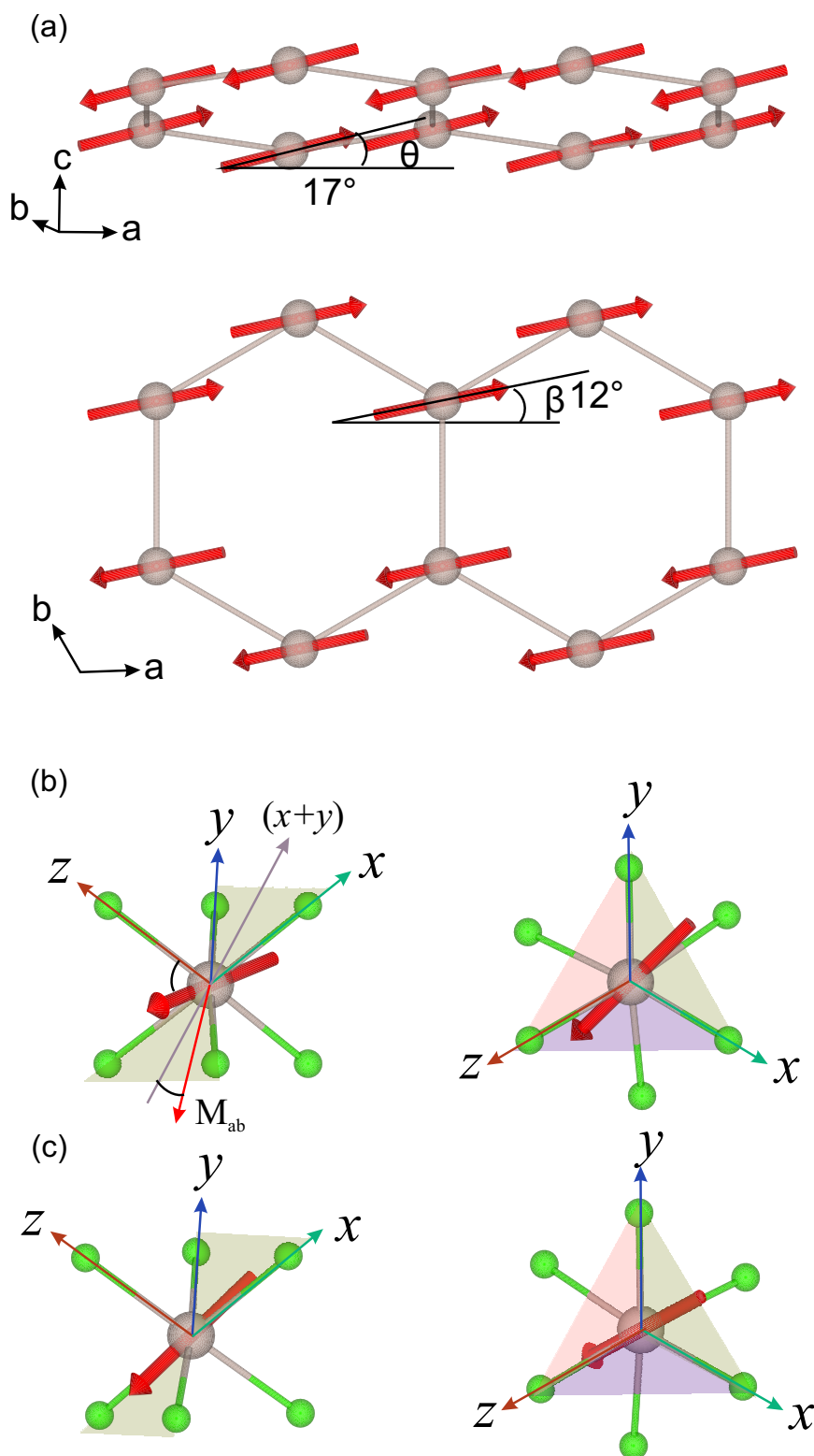
Figure 5.11: (a) Illustration of magnetic structure refined from the spherical neutron polarisation data at 1.5 K obtained from IN12. (b) and (c) the direction Magnetic moment of Ru 3+ are depicted in a local rectangular coordination xyz for model I and model II and III. This local coordinate system has been introduced in Fig.2.13.
