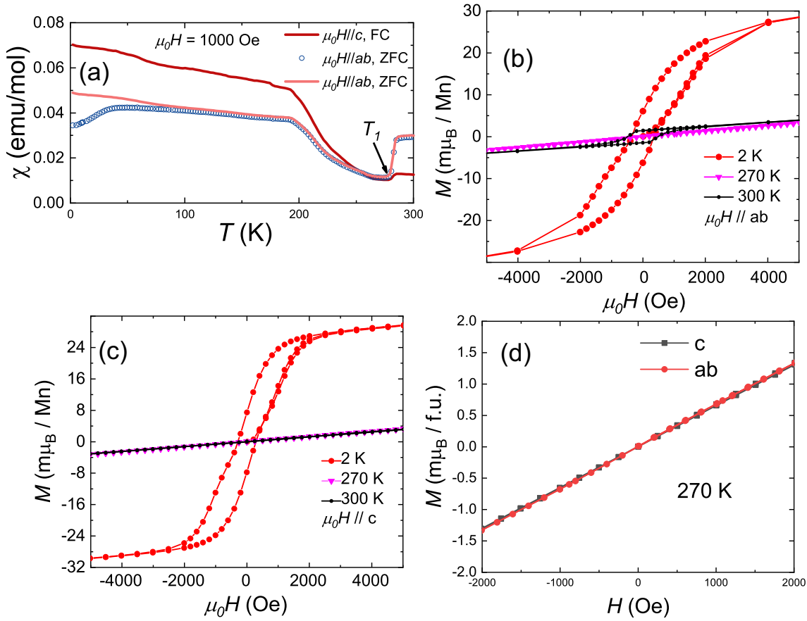
Figure 4.6: Magnetic properties of Mn_3Sn single crystals. (a) Temperature dependence of magnetic susceptibility measured in Mn_3Sn ab basal plane and c direction under a magnetic field of 1000 Oe in field cooling (FC) and zero field cooling (ZFC) conditions. (b) and (c) Isothermal magnetization of ab plane and c direction measured at 300 K, 270 K and 2 K. (d) Comparison of isothermal magnetization of ab plane and c direction at 270 K.
