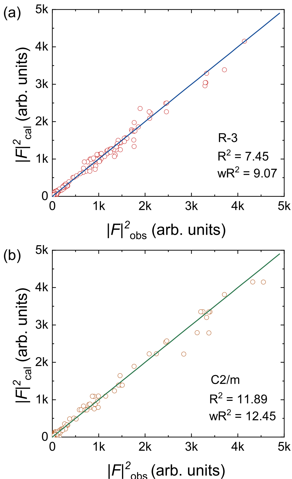
Figure 5.7: Calculated square of structure factors |F|_{\text{cal}}^2 versus observed square of structure factors |F|_{\text{obs}}^2 in R\bar{3} in C2/m and R\bar{3} models. |F|_{\text{obs}}^2 was obtained from the single crystal neutron diffraction measurements at T = 2 K. (a) Observed square of structure factor square |F|_{\text{obs}}^2 versus calculated ones for R\bar{3} structure model. (b) Observed square of structure factor square |F|_{\text{obs}}^2 versus calculated |F|_{\text{cal}}^2 for C2/m structure model.
