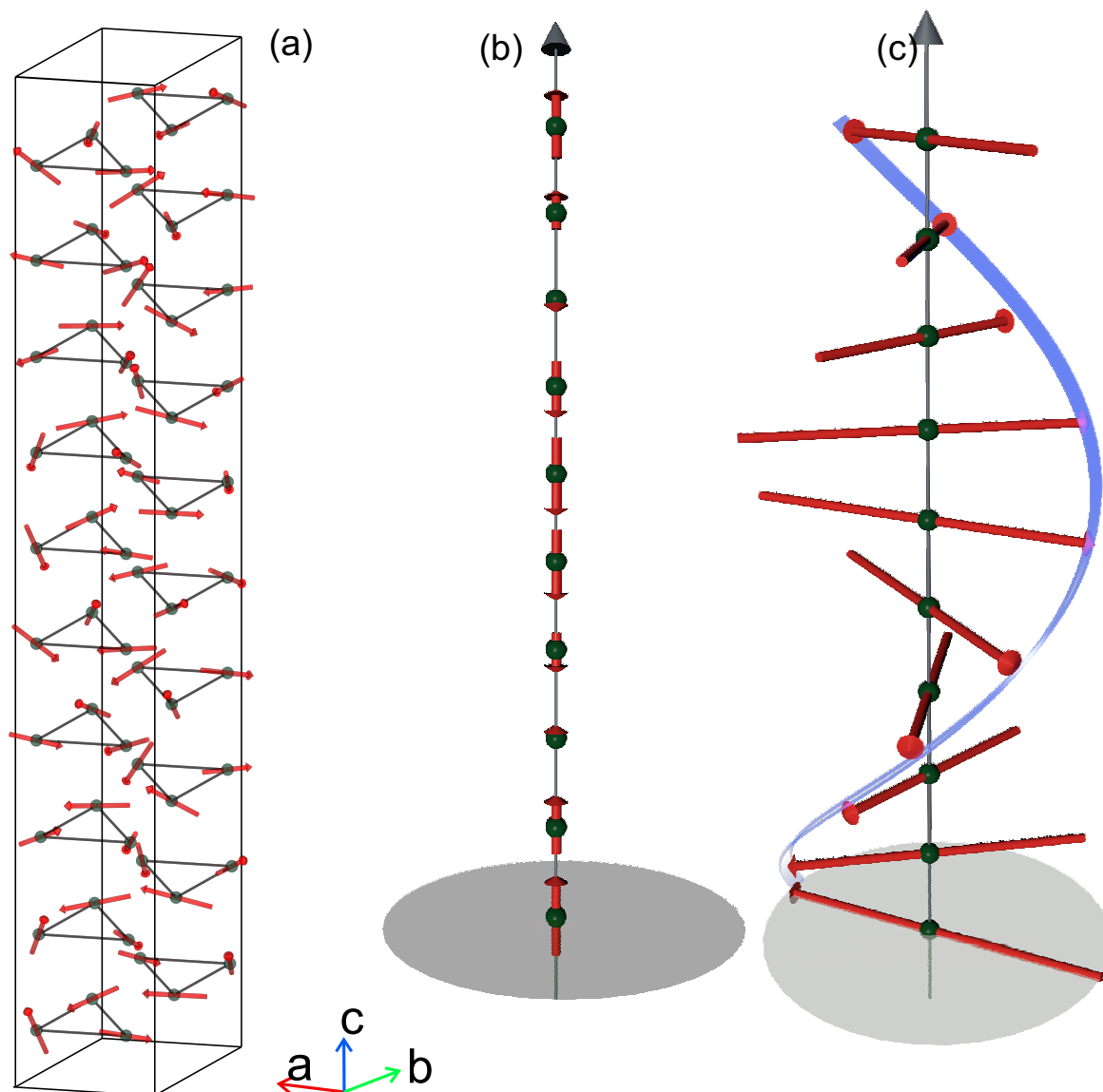
Figure 4.18: Refined magnetic structure from single crystal neutron diffraction data of Mn_3Sn at 225 K collected at HEiDi at MLZ. (a) Superstructure of Mn_3Sn with ten Mn_3Sn unit cells, where only Mn atoms are plotted. Magnetic structure model is plotted by Vesta [62]. (b) The magnetic components along c direction are a longitudinal spin density wave, which are measured in zn\bar{s}f channels. (c) The magnetic components lying in ab plane are a helix, which are measured in z\bar{s}f channels.
