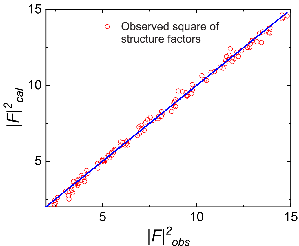
Figure 4.4: Refined square of structure factors versus calculated square of structure factors of the pure nuclear reflections for the Mn_3Sn from single crystal neutron diffraction data at 210 K collected at HEiDi at MLZ.
