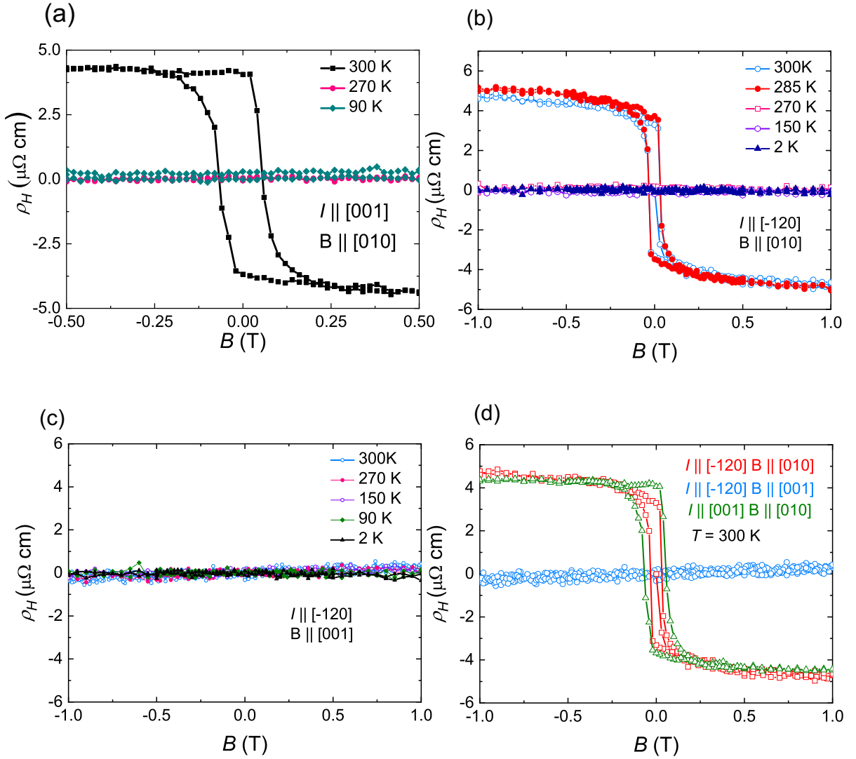
Figure 4.8: Magnetic field dependence of Hall effects in Mn_3Sn . (a) Measured with the electric current along [0,0,1] and magnetic field along [0,1,0] under various temperatures. (b) Measured with the electric current along [\bar{1},2,0] and magnetic field along [0,1,0] under various temperatures. (c) Measured with the electric current along [\bar{1},2,0] and magnetic field along [0,0,1] under various temperatures. (d) Comparison of AHE among three above measured conditions at 300 K.
