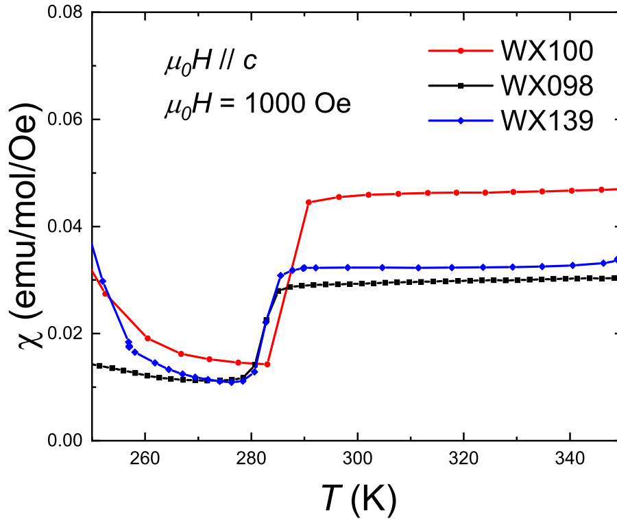
Figure 4.5: Comparison of magnetic susceptibility of Mn_3Sn from different batches measured for field along c direction under zero field cooling condition, where a phase transition is observed at \sim 280 K.
