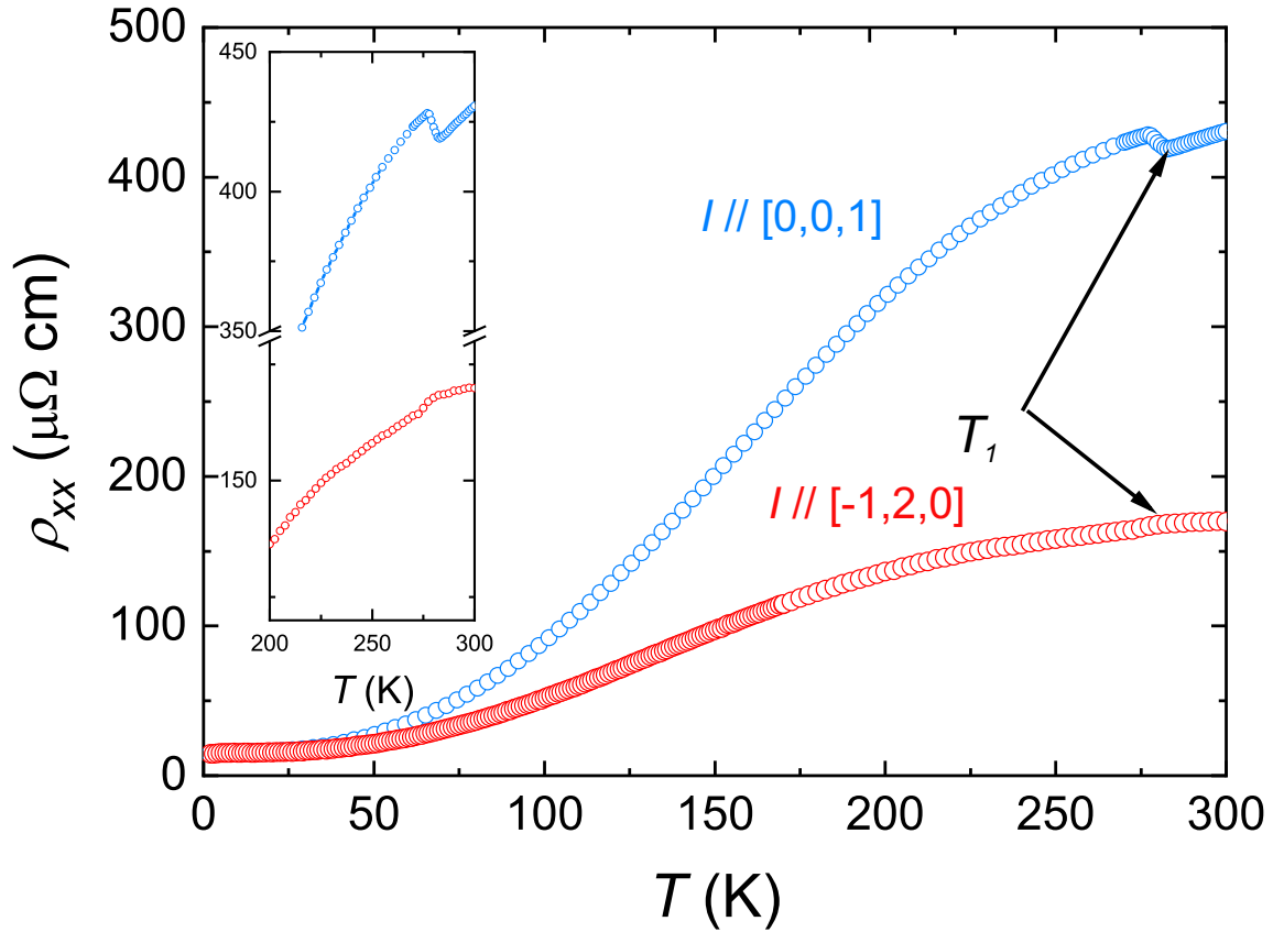
Figure 4.7: Temperature dependence of longitudinal electrical resistivity \rho_{xx} of the Mn_3Sn as-grown single crystal with current applied along [0,0,1] and [\bar{1},2,0] at zero field.
