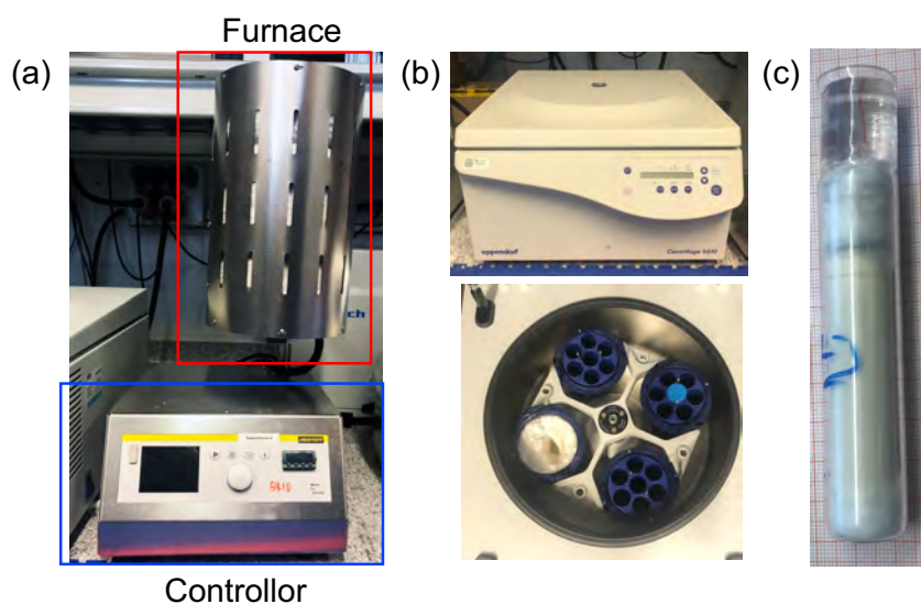
Figure 3.2: Equipments of the crystal growth from the flux method in this PhD work. (a) Tube furnace with working temperature from room temperature to 1200^\circ\text{C} manufactured by Nabertherm. (b) Centrifuge. (c) A sealed silica ampoule with samples inside.
